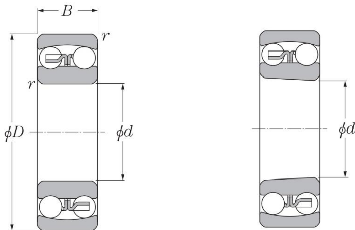
Cylindrical bore
