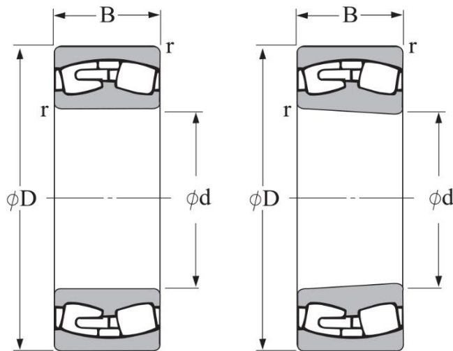
Cylindrical Bore
